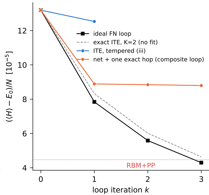
(c) guide energy (Krylov sign)
