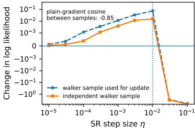
(b) 8 x 8: SR step, held-out walkers
