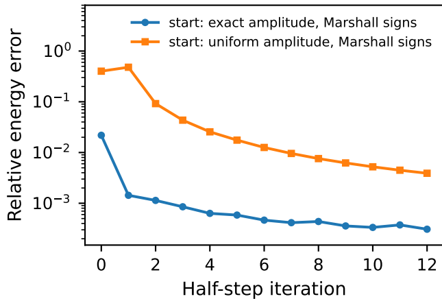
(a) 4 x 4: exact half-step target
