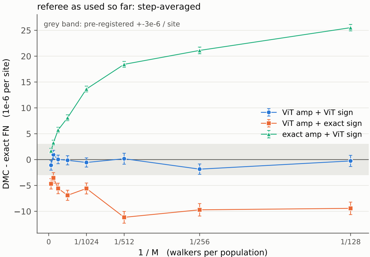
Lattice FN referee vs exact symmetric-sector FN, 6x6 J1-J2 ( J_2/J_1 = 0.5 ), \tau_{\max} = 0.025 , beta window 0.8-2.4
