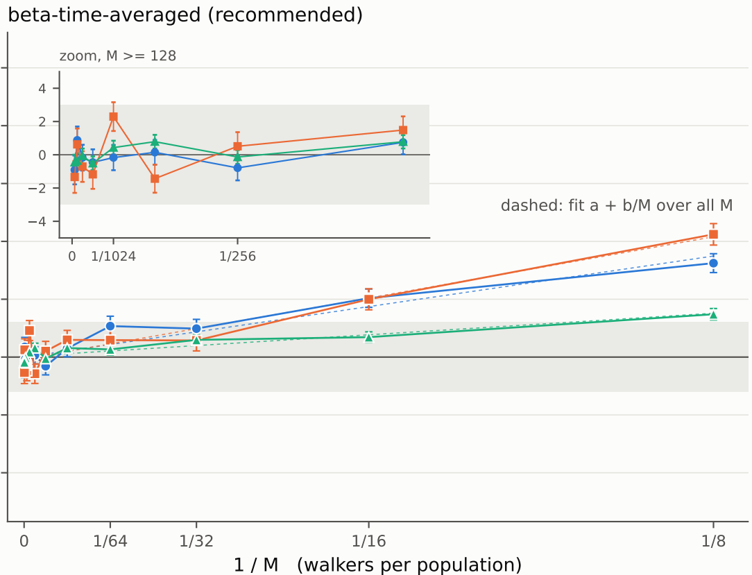
Lattice FN referee vs exact symmetric-sector FN, 6x6 J1-J2 ( J_2/J_1 = 0.5 ), \tau_{\max} = 0.025 , beta window 0.8-2.4
