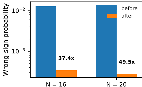
(c) J_2 / J_1 = 0.5 , exact
