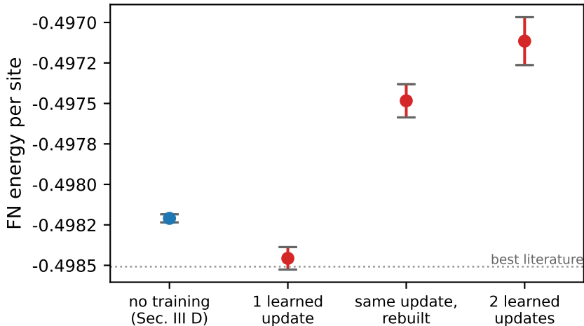
8 x 8, J_2 / J_1 = 0.5 : learned amplitude updates
