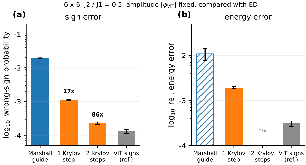
FIG. 4. Krylov sign steps on the ViT amplitude ( 6 \times 6 ), compared with ED, with the ViT's own signs as reference. (a) Wrong-sign probability ( 4 \times 10^5 exact samples). (b) Relative energy error; the Marshall value (hatched) is a lower bound from a smaller sample, the two-step energy is not resolved.
