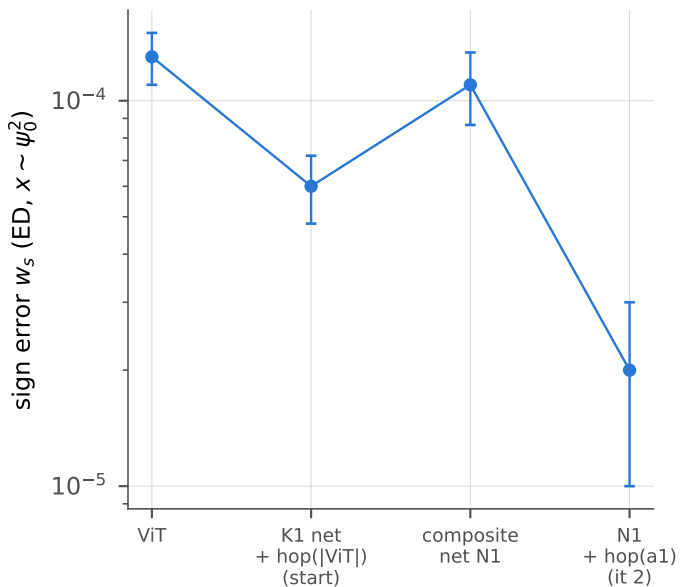
(a) Signs: composite net + one hop
