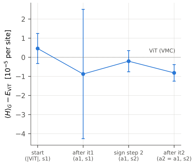
(b) Guide energy vs ViT (paired)
