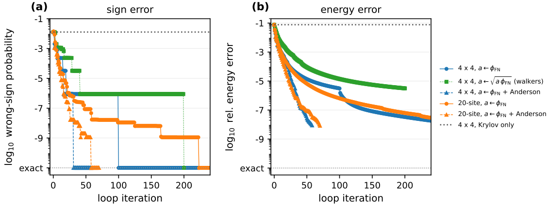
FIG. 5. Fixed-node-Krylov loop with exact diagonalization, started from the J_2 = 0 amplitude with Marshall signs, for three amplitude updates: a \leftarrow \phi_{\text{FN}} ; a \leftarrow \sqrt{a} \phi_{\text{FN}} , as learned from walkers; and a \leftarrow \phi_{\text{FN}} with Anderson extrapolation from the last three iterates. Dotted: Krylov steps alone from the same start, which change no sign. (a) Sign and (b) energy error vs iteration, compared with ED. All values are exact (no statistical error).
