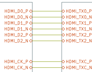
FPGA_HDMI
