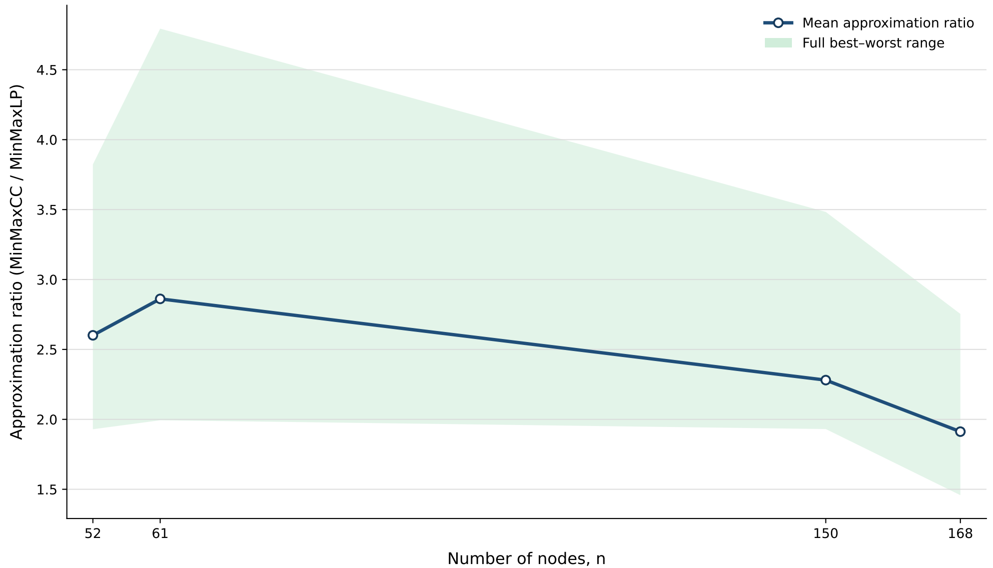
MinMaxCC approximation ratio by Facebook graph size
