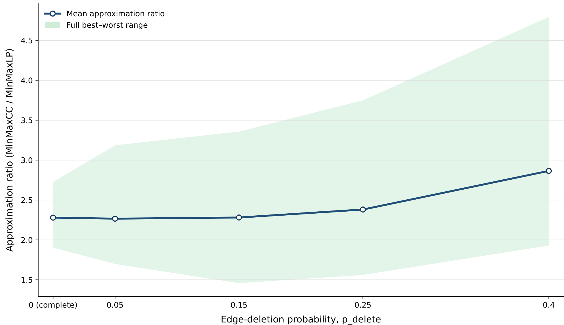
MinMaxCC approximation ratio by edge-deletion probability
