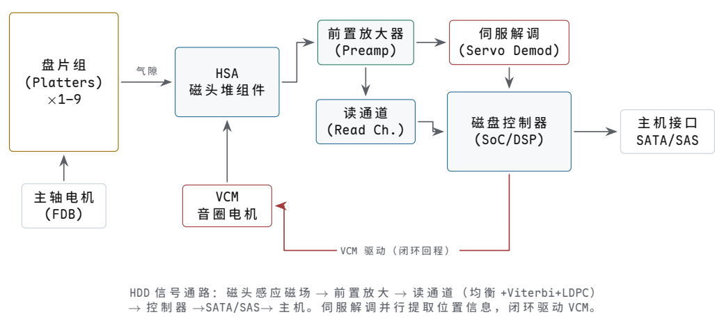
图示：HDD 整机框图。读路径（左 → 右）：磁头 → Preamp → Read Channel → Controller → Host。伺服路径：Preamp → Servo Demod → Controller → VCM Driver → VCM。写路径反向：Controller → Write Channel → Preamp → 磁头。
