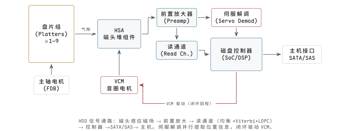
图示：HDD 整机框图。读路径（左 → 右）：磁头 → Preamp → Read Channel → Controller → Host。伺服路径：Preamp → Servo Demod → Controller → VCM Driver → VCM。写路径反向：Controller → Write Channel → Preamp → 磁头。
