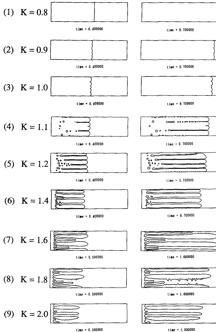
Fig. 6. Crystal grows from the left wall toward supercooled melt under adiabatic condition for various values of K . There is 4-mode anisotropy. \delta = 0.050 .
