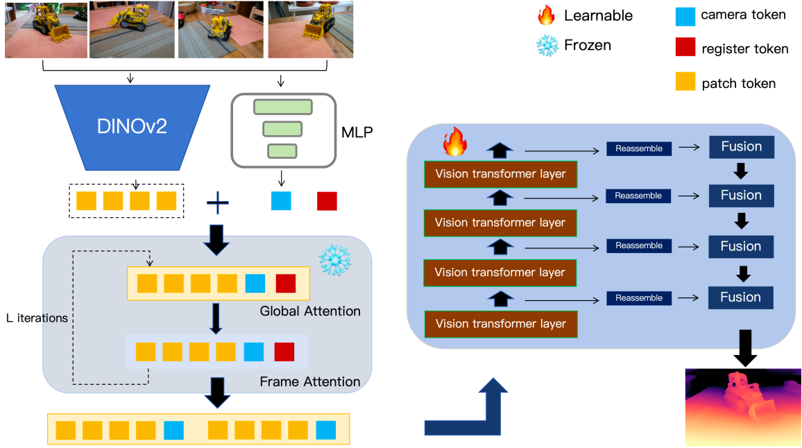
Figure 2. VGGT-Depth prior used for depth-guided point cloud densification.
