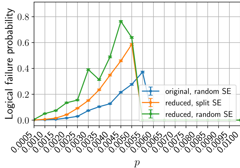
Heawood Cycle
