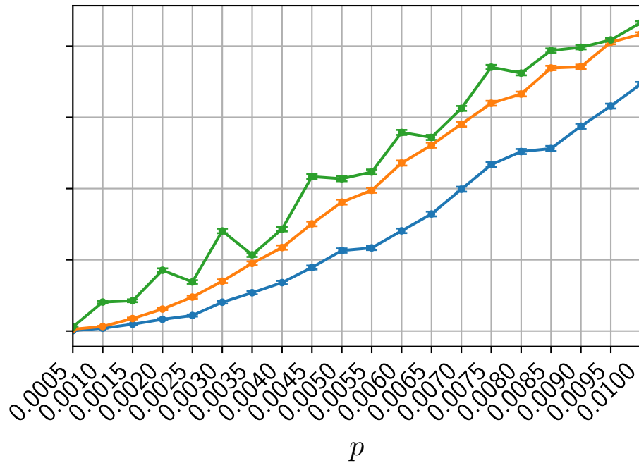
K33 Cycle
