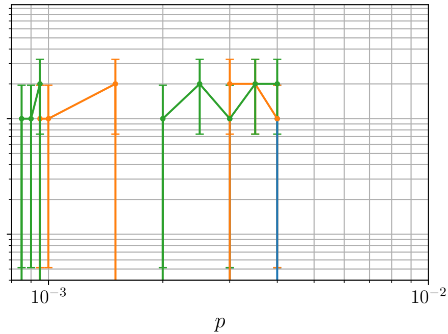
K_33
