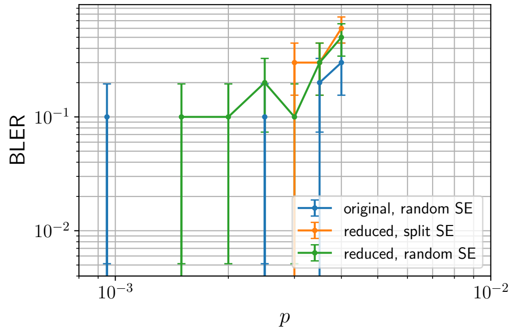
heawood
