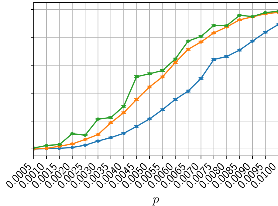
Petersen Cycle
