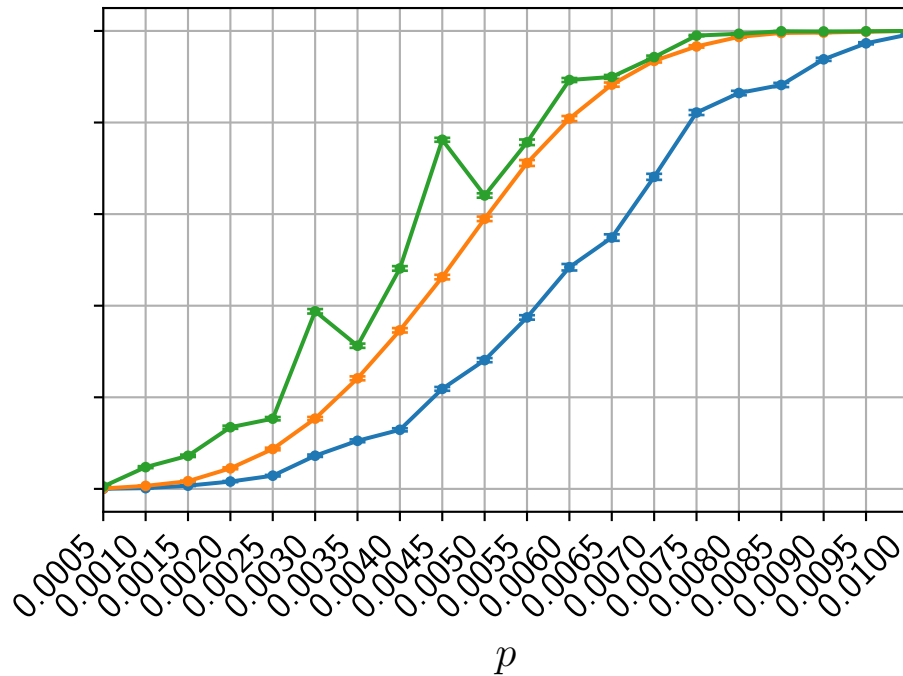
Heawood Cycle
