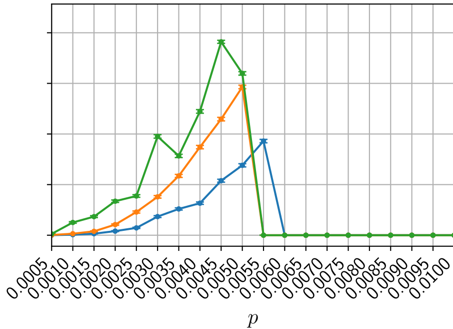
Heawood Cycle
