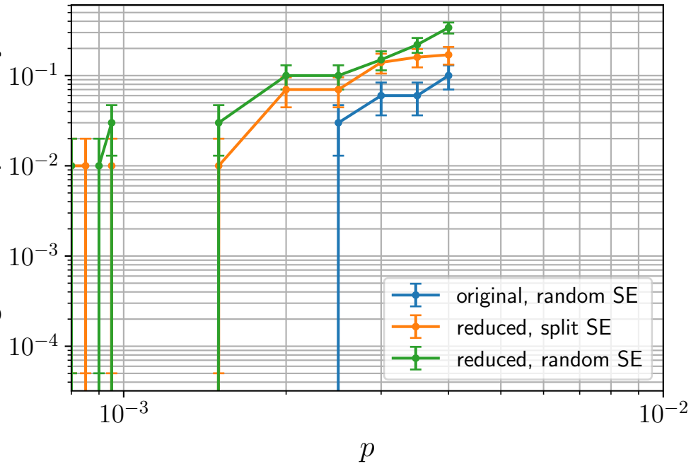
Petersen Cycle
