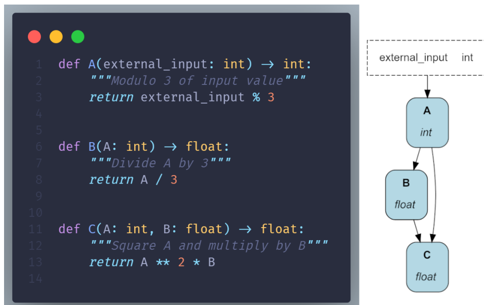
The ABC of Apache Hamilton
