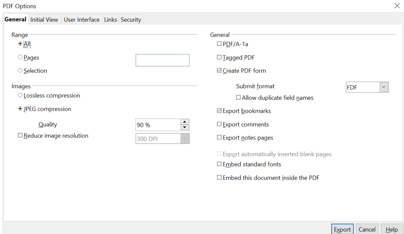
Figure 196: General tab of PDF Options dialog
