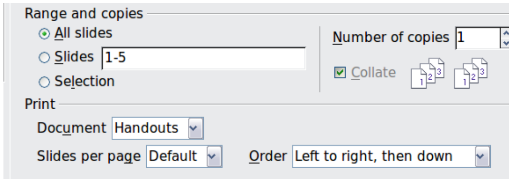
Figure 194: Printing handouts
