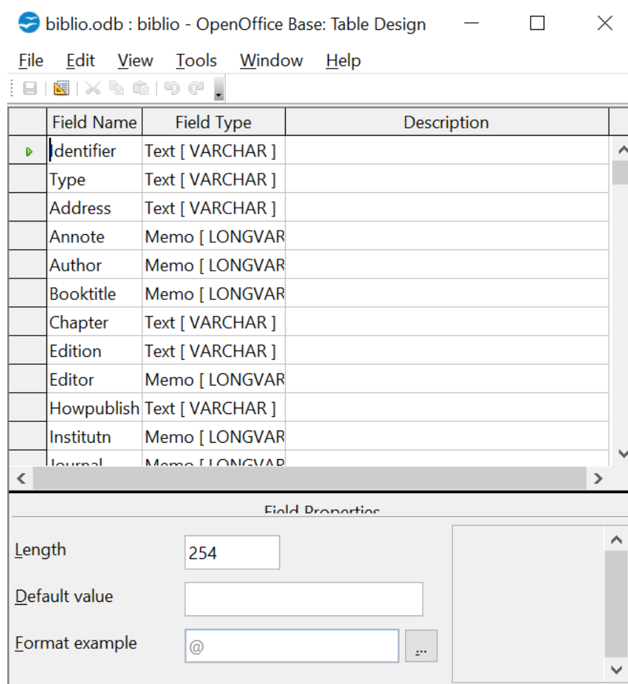
Figure 23. Modify table properties window
