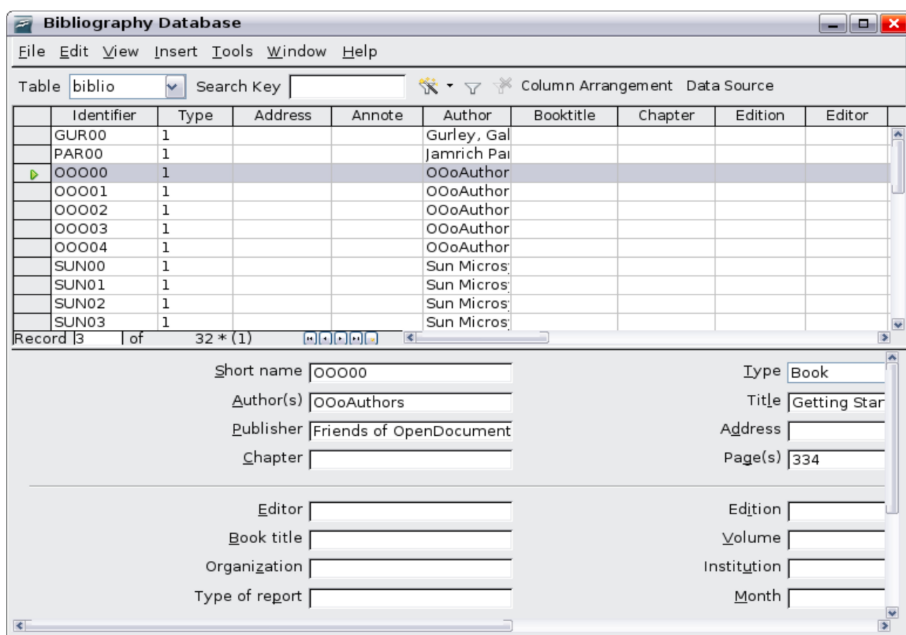
Figure 17. Bibliography Database main window
