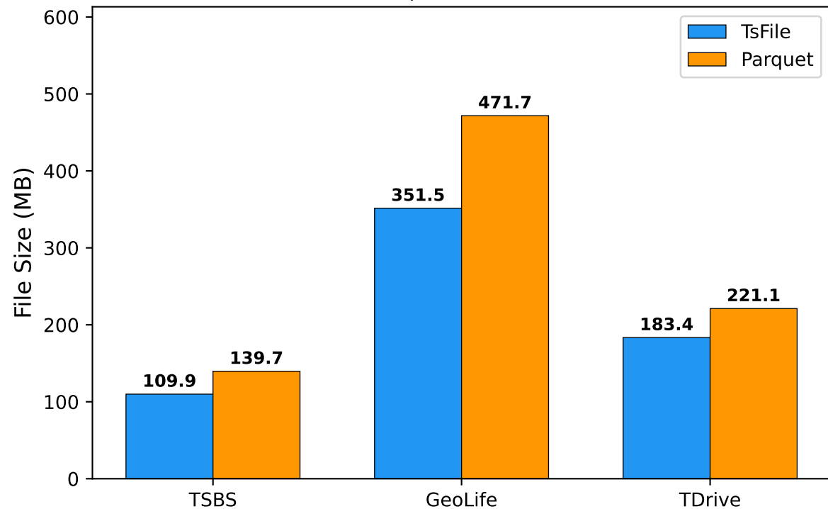
Space Cost
