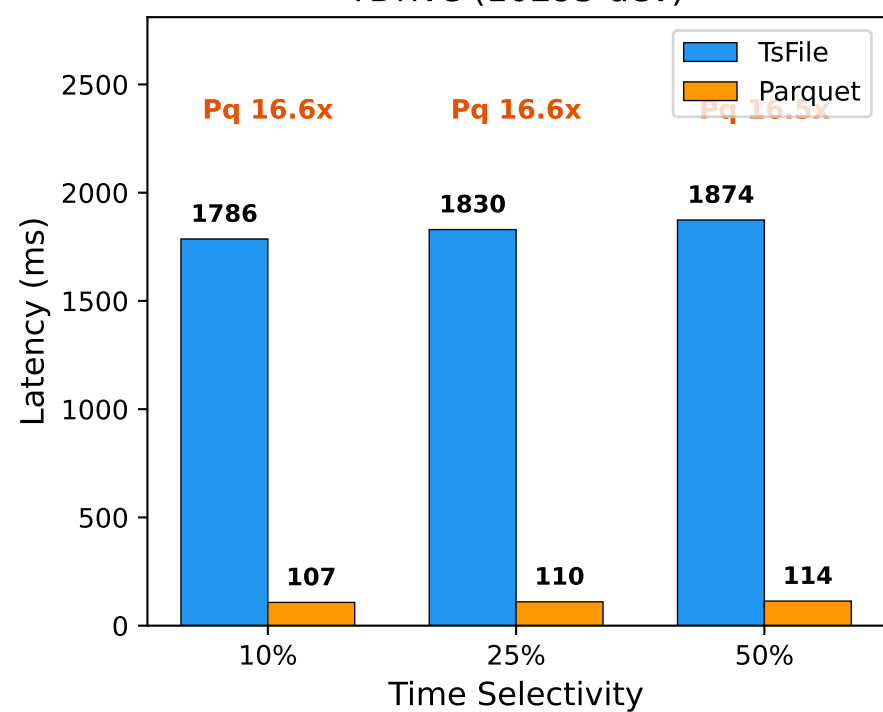
TDrive (10295 dev)
