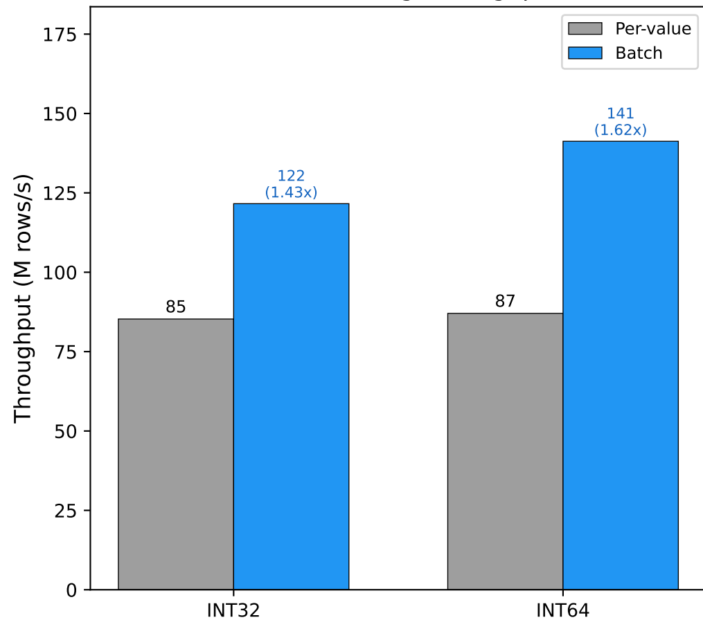
T5-1: Encoding Throughput
