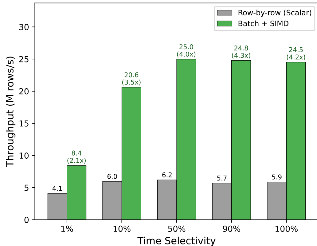
End-to-End Read Throughput
