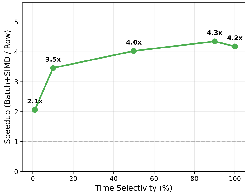
Speedup vs Selectivity
