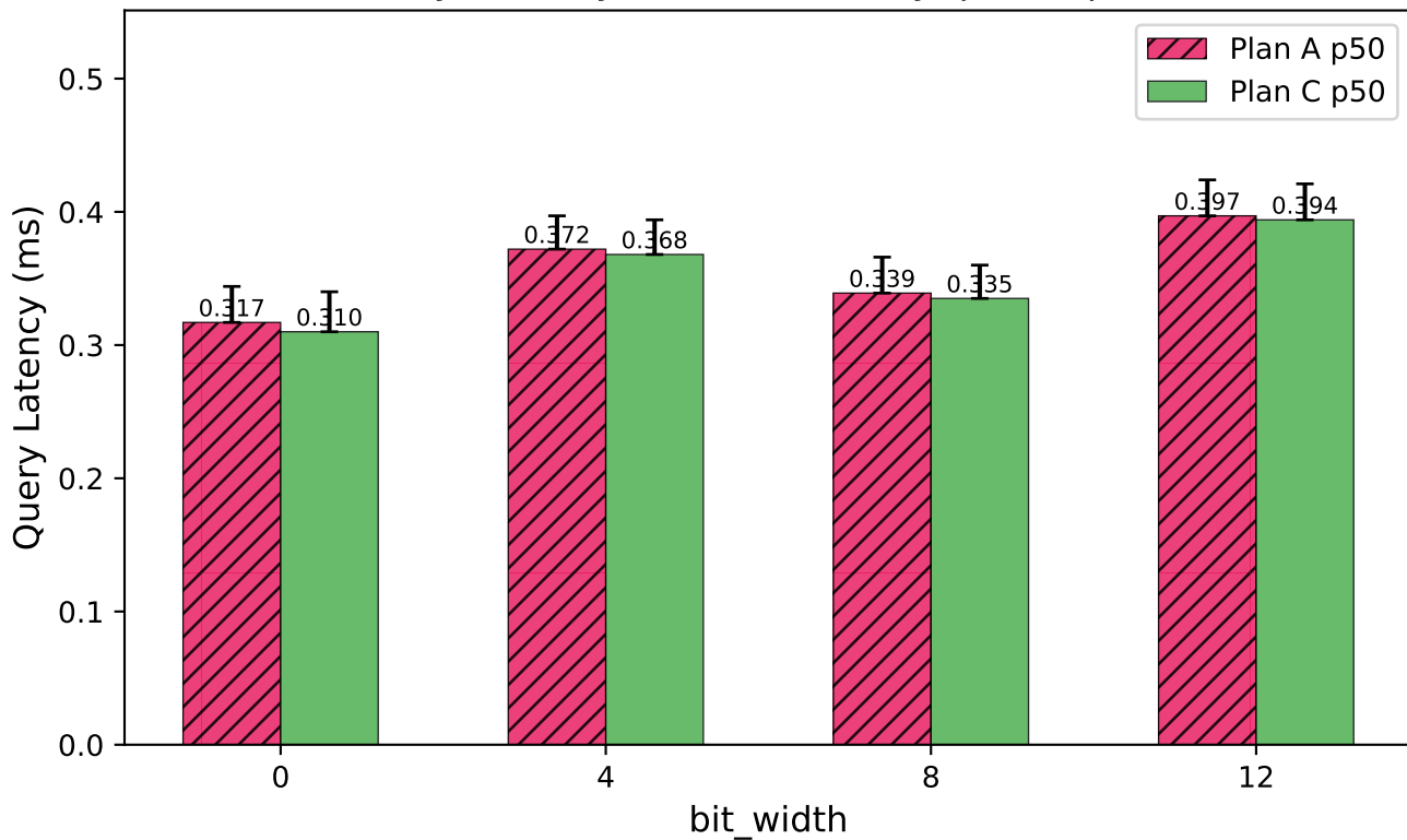
E5-4b: Query Latency (10% selectivity, p50 + p95 whisker)
