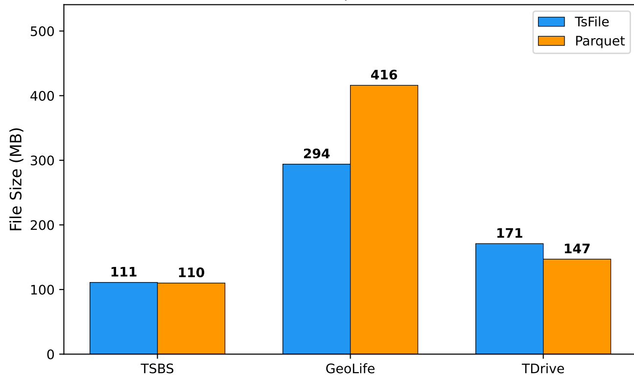
T6-1a: Space Cost
