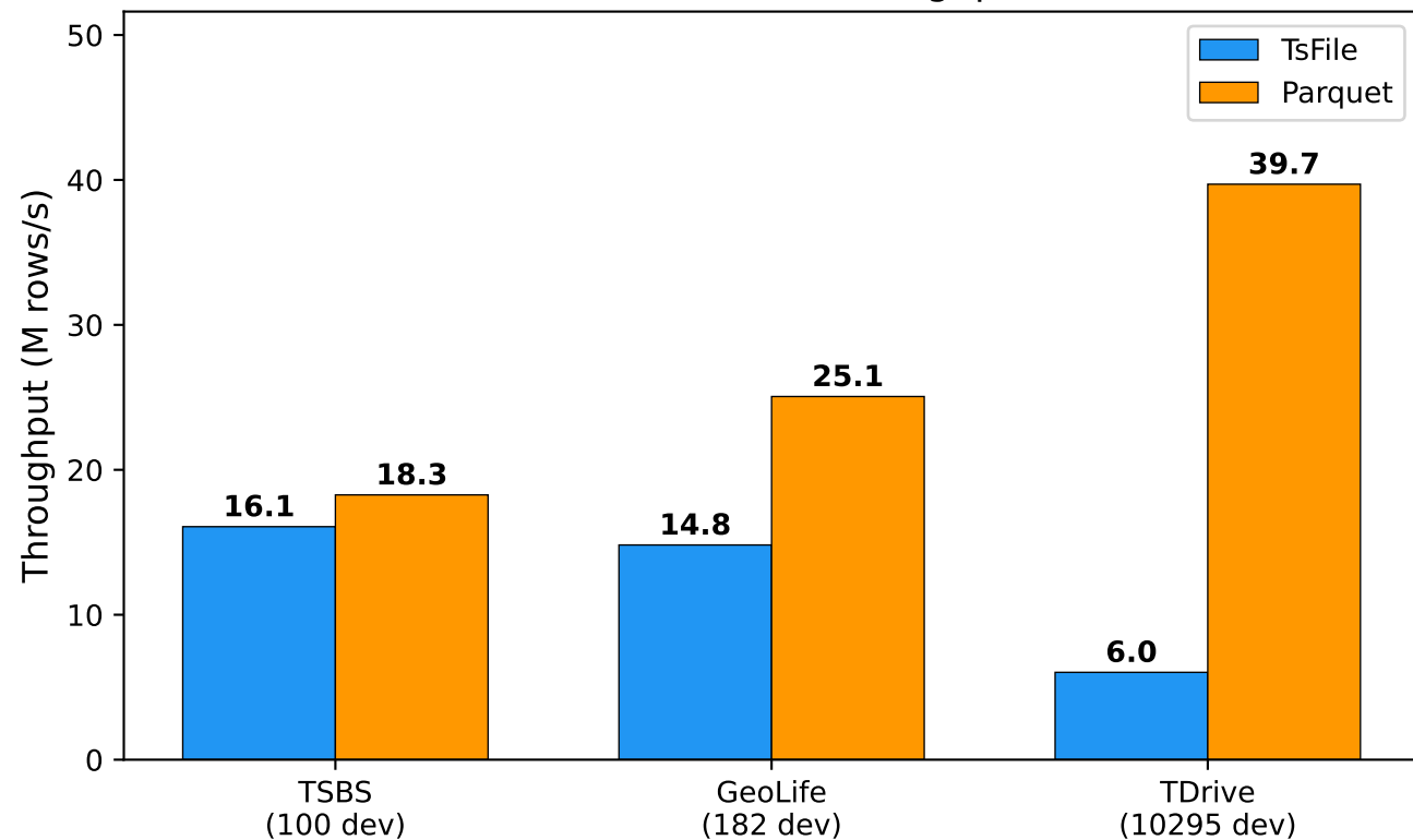
T6-1c: Full Scan Throughput
