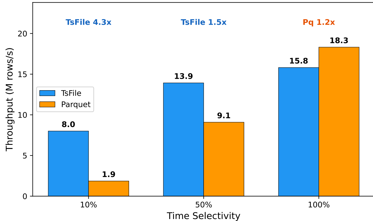
T6-1d: Time Filter Throughput (TSBS, 100 devices)
