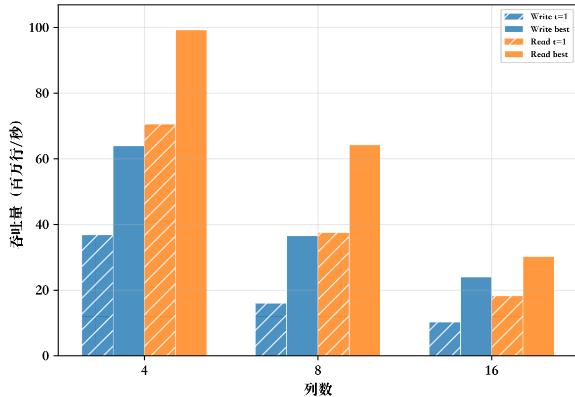
SNAPPY
