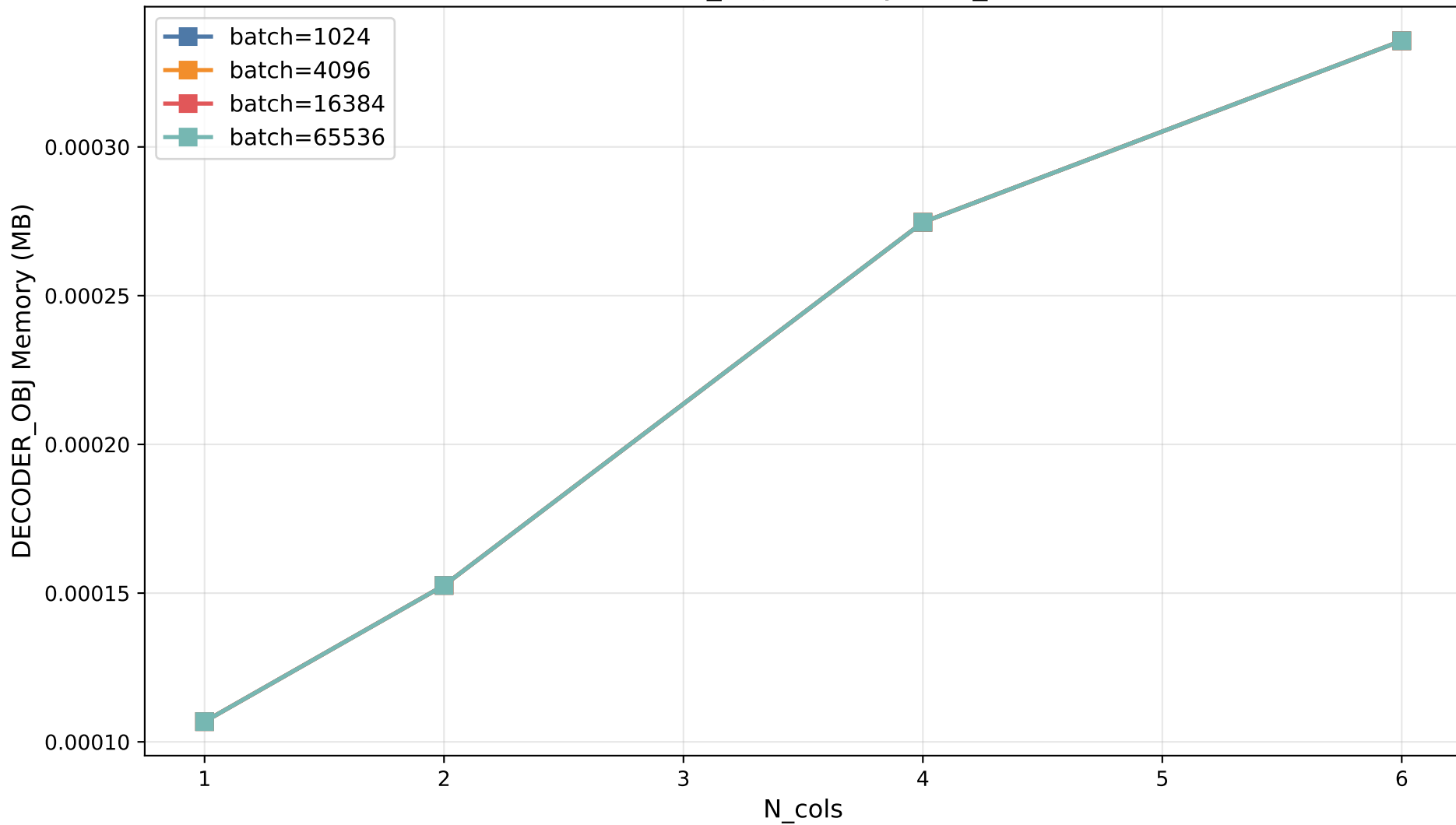
DECODER_OBJ Memory vs N_cols
