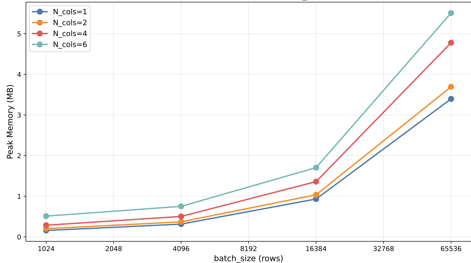
Peak Total Memory vs batch_size
