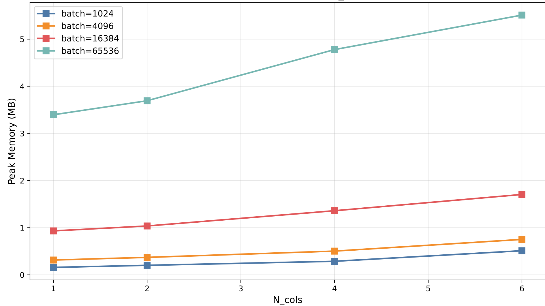
Peak Total Memory vs N_cols
