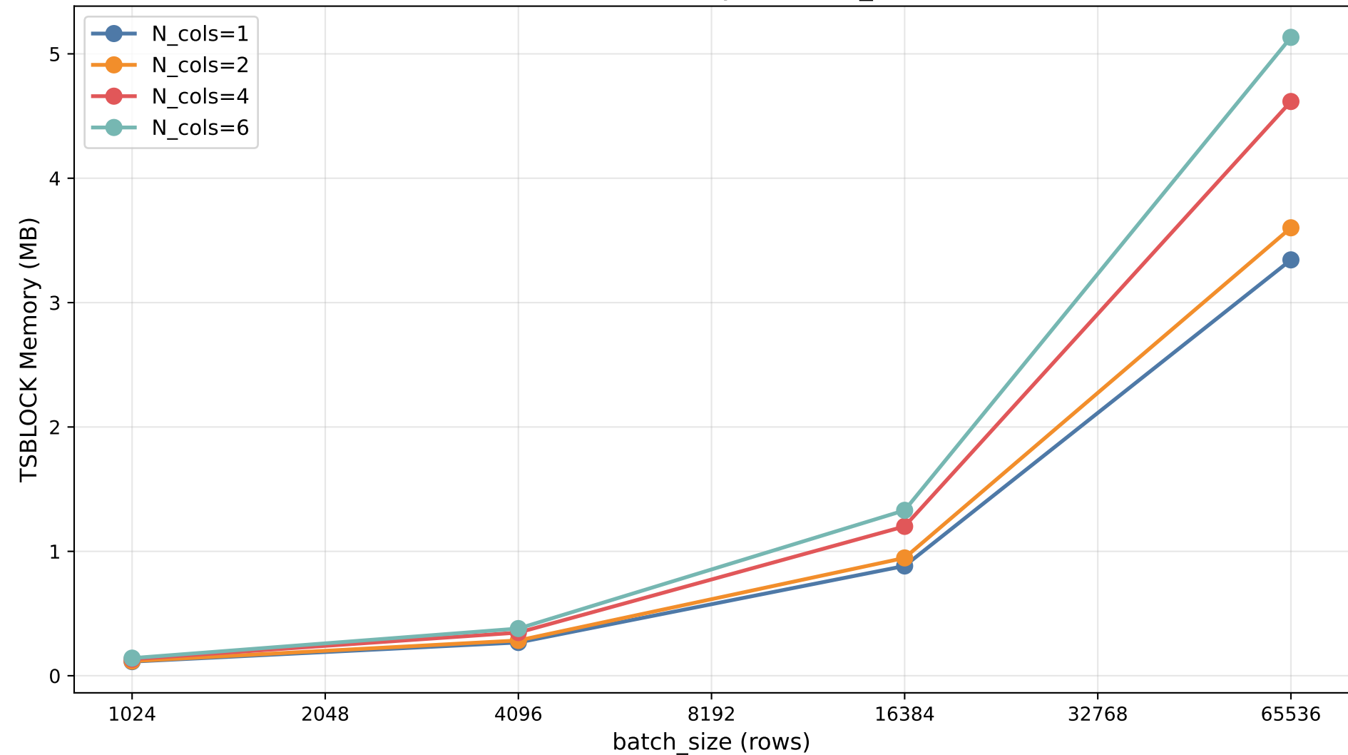
TSBLOCK Memory vs batch_size
