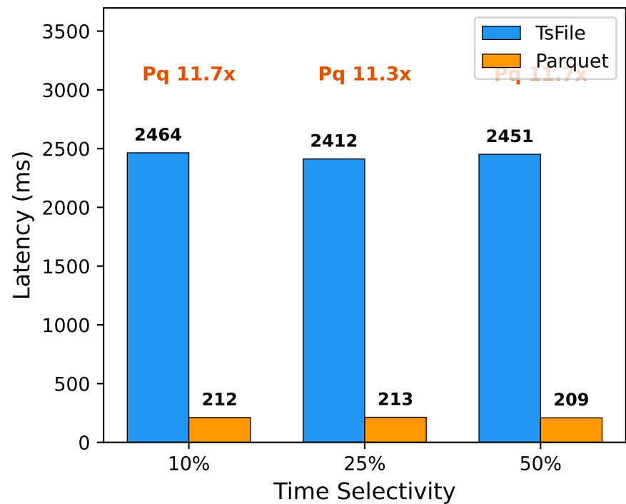
TDrive (10295 dev)
