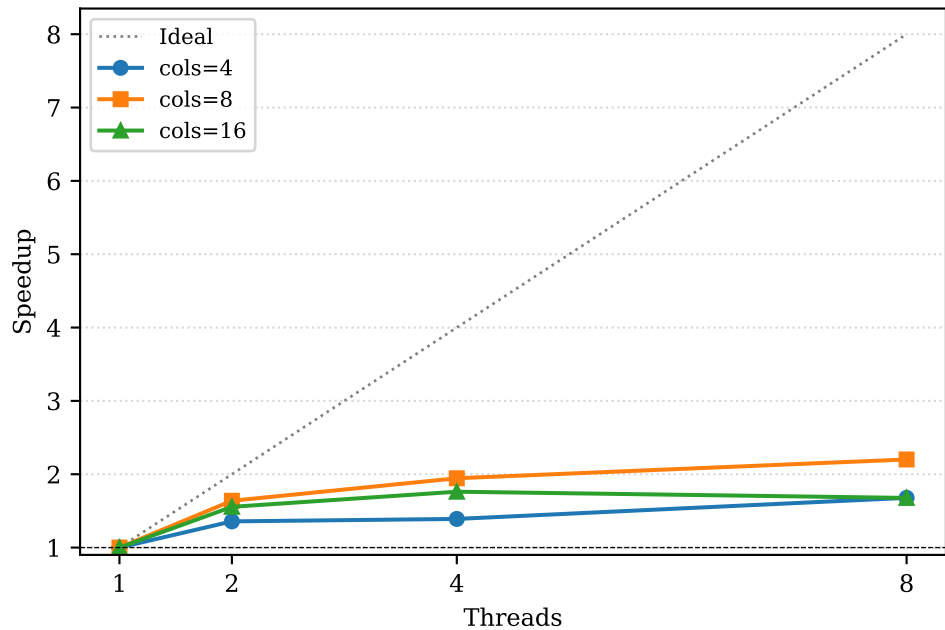
SNAPPY
