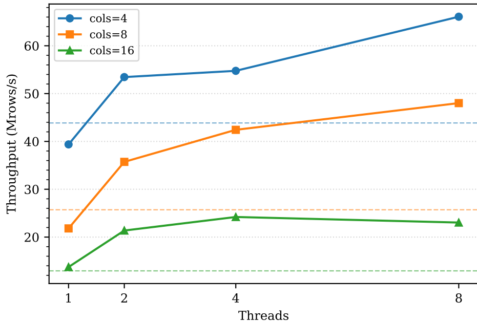
SNAPPY
