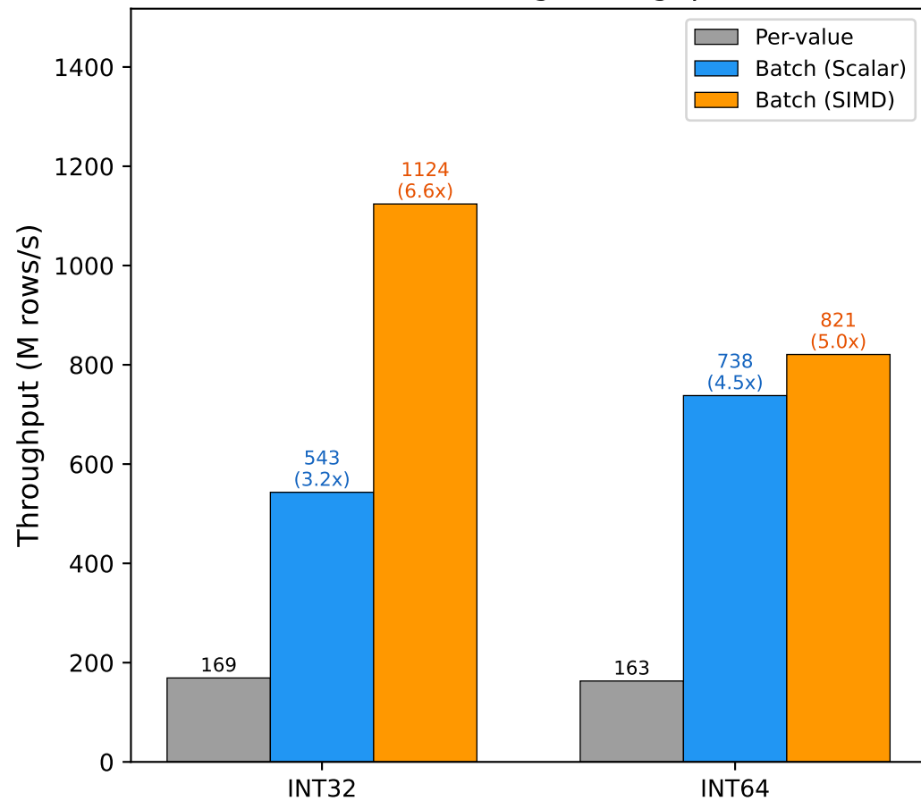
T5-2: Decoding Throughput
