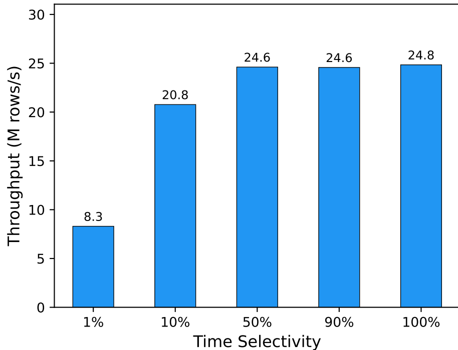
F5-1: Read Throughput vs Selectivity
