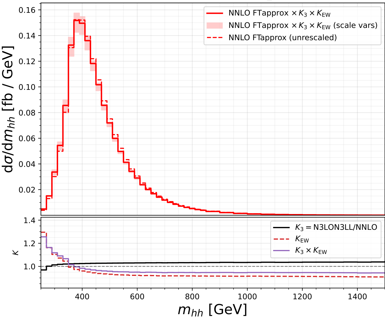
m_{hh} distribution, \sqrt{s} = 13 TeV, PDF4LHC21_40, m_h = 125 GeV
