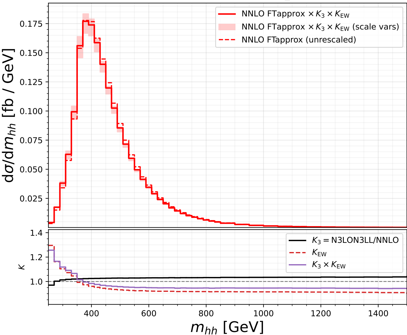
m_{hh} distribution, \sqrt{s} = 14 TeV, PDF4LHC21_40, m_h = 125 GeV
