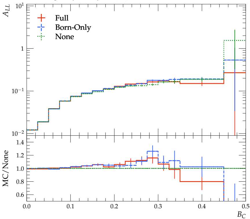
Double-spin asymmetry A_{LL}(B_C)
