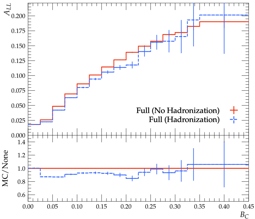
Double-spin asymmetry A_{LL}(B_C)
