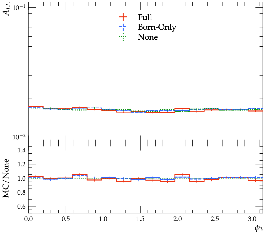
Double-spin asymmetry A_{LL}(\phi_3)
