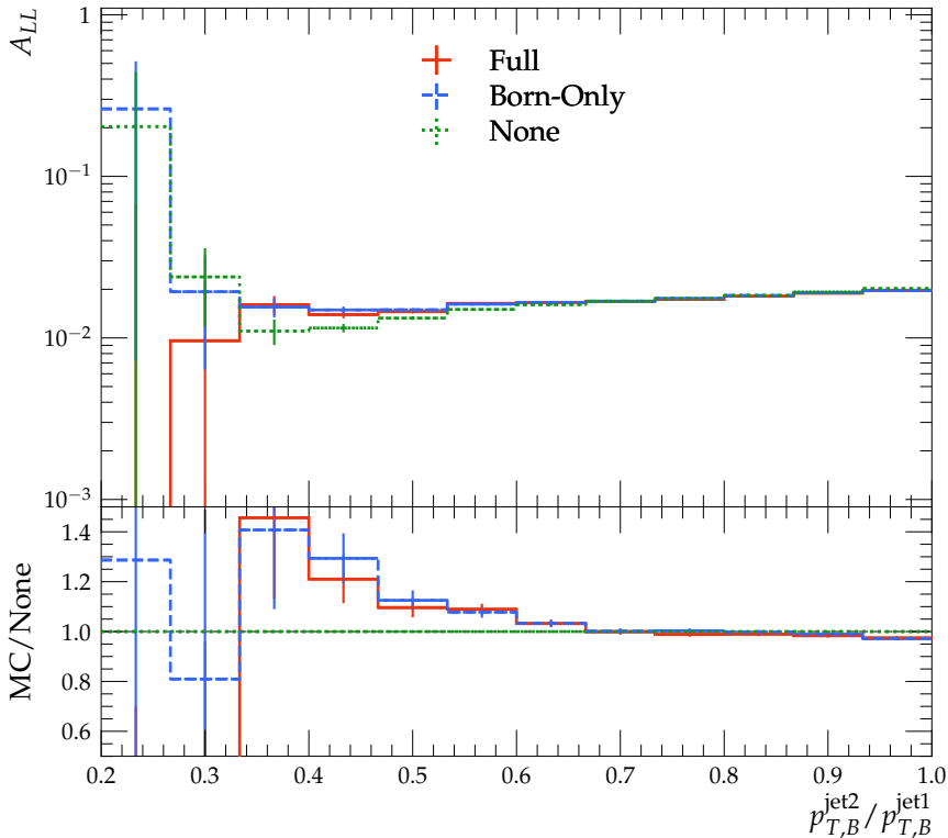
Double-spin asymmetry A_{LL}(p_{T,B}^{\text{jet2}}/p_{T,B}^{\text{jet1}})
