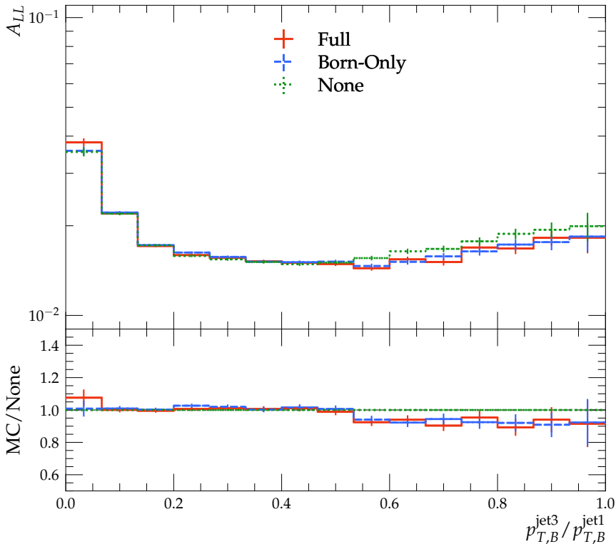
Double-spin asymmetry A_{LL}(p_{T,B}^{\text{jet3}}/p_{T,B}^{\text{jet1}})
