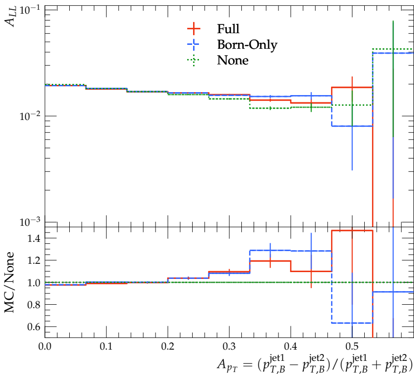
Double-spin asymmetry A_{LL}(A_{p_T})
