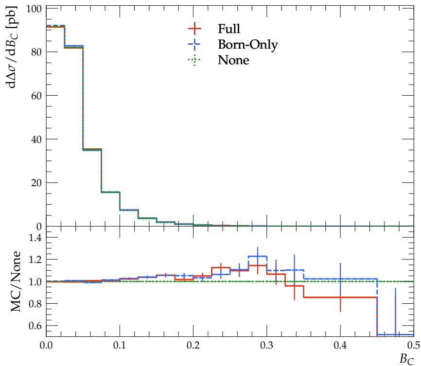
Polarized current-hemisphere broadening d\Delta\sigma/dB_C
